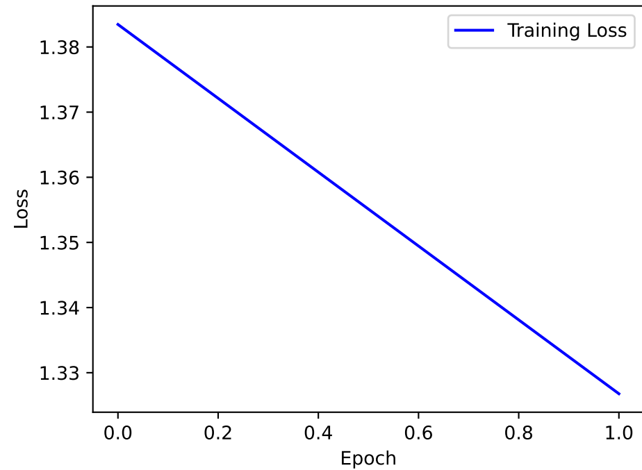
Training Loss
