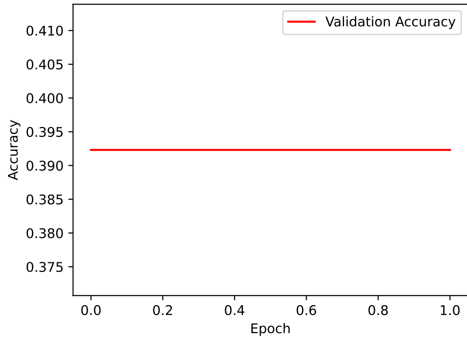
Validation Accuracy
